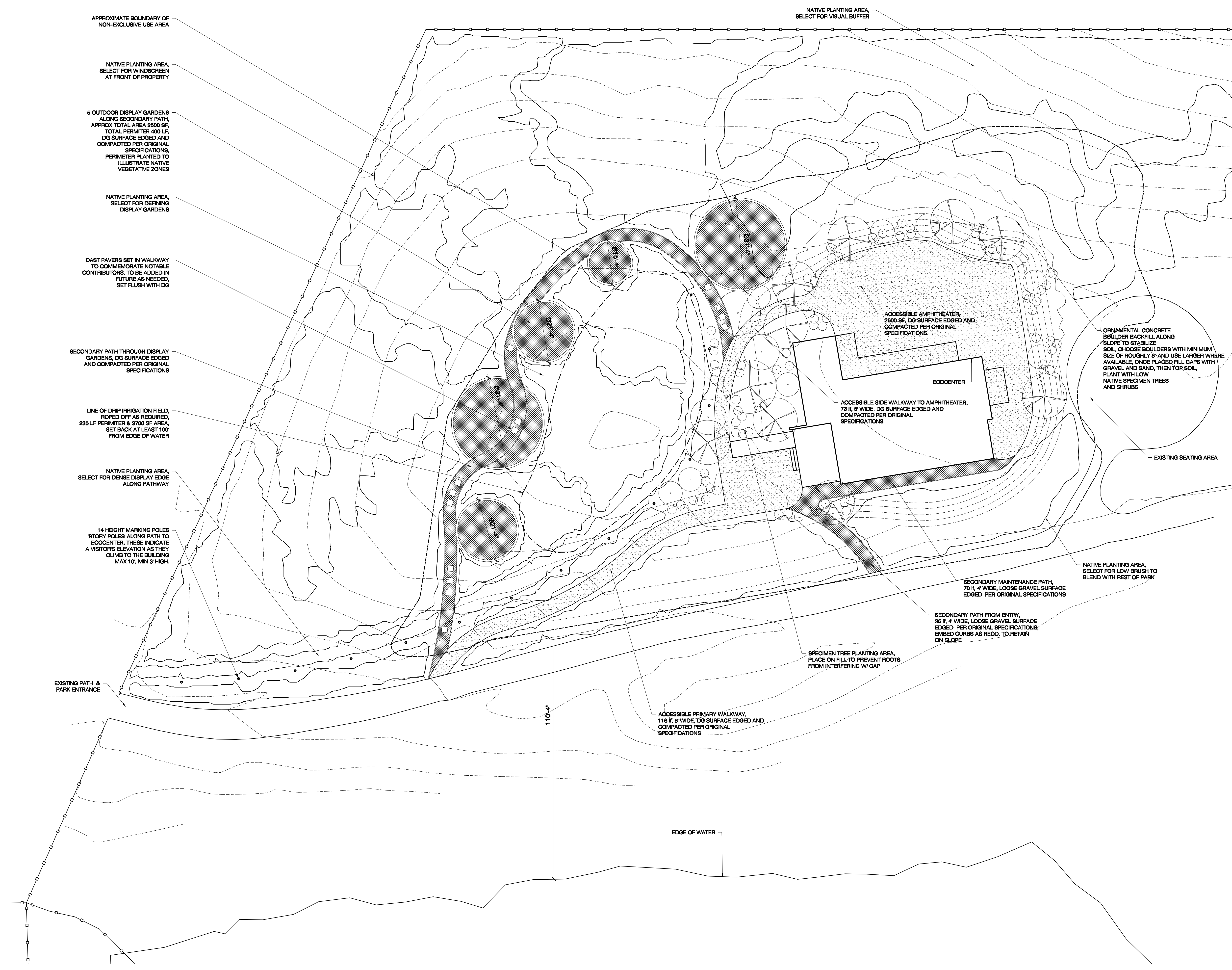
1 PROPOSED SITE LANDSCAPE PLAN 1/16" = 1'-0"
